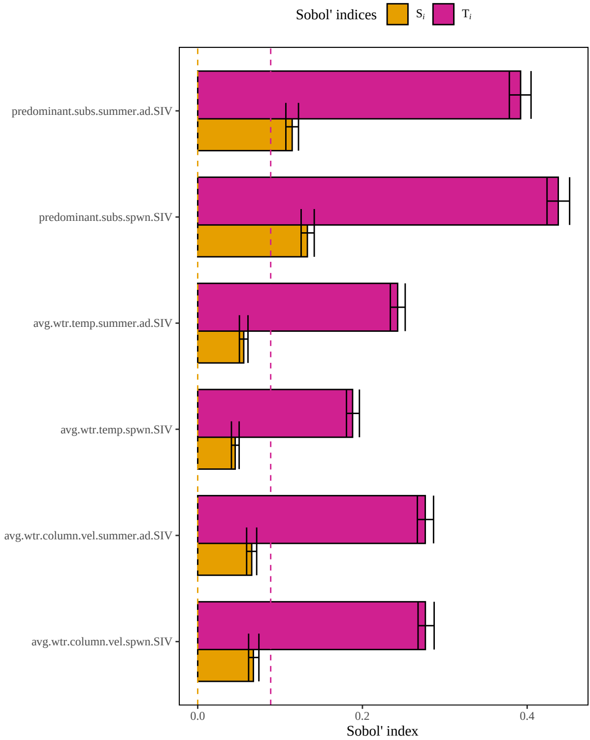
Figure 7. Results of a sensitivity analysis for the shortnosesturgeon model based on a multiplicative mean structure. Dashed lines represent baseline numerical approximation error for S_i and T_i ( i.e. , dummy variables).
